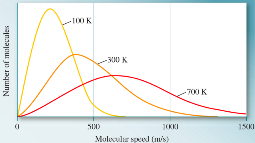
N 2 (28.02 g/mol)
